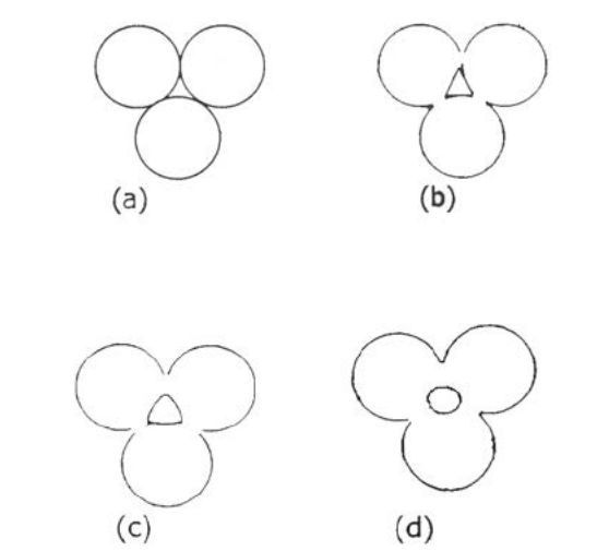
Fig: Schematic illustration of three sphere sintering model: (a) original point contacts (b) and (c) neck growth (d) pore rounding. (From J.S Hirschhorn, introduction to powder Metallurgy Institute, New York, 1967.)
